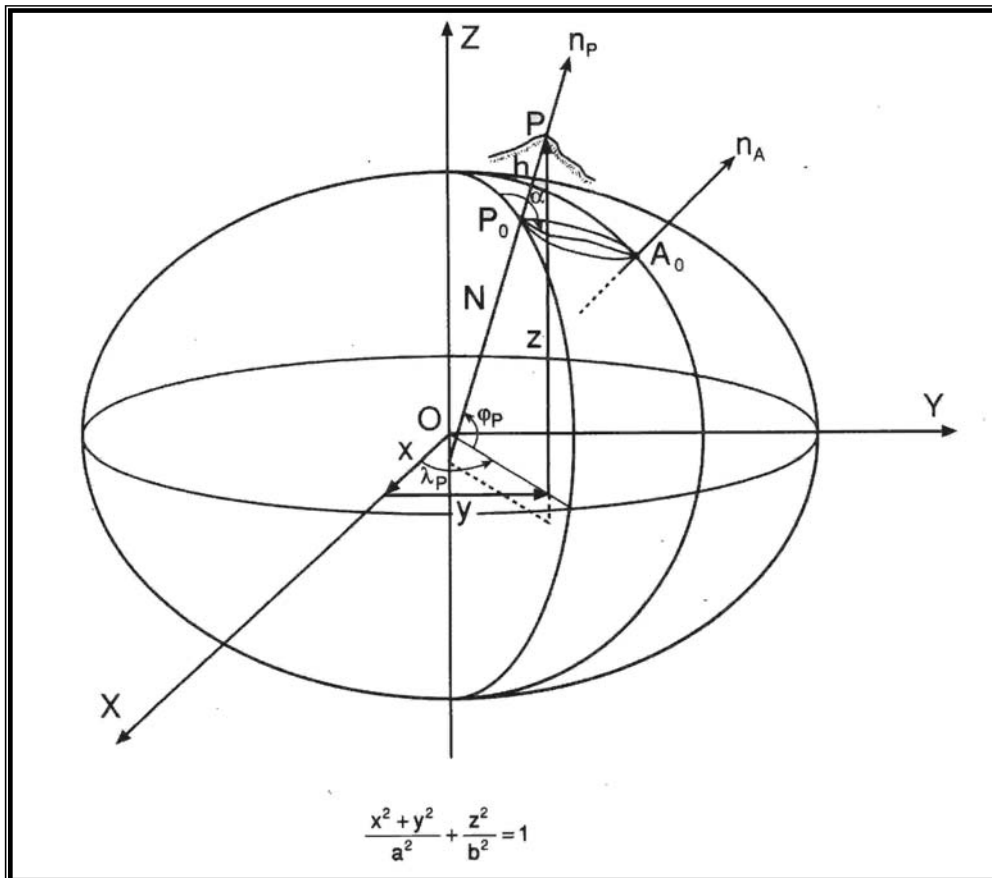
Fig. 2.2 "The Ellipsoid"
