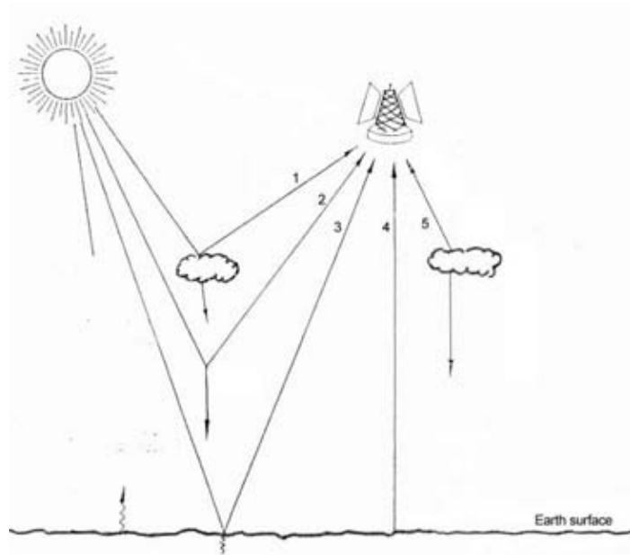
Fig. 6.36 "Radiation received by the sensors"
