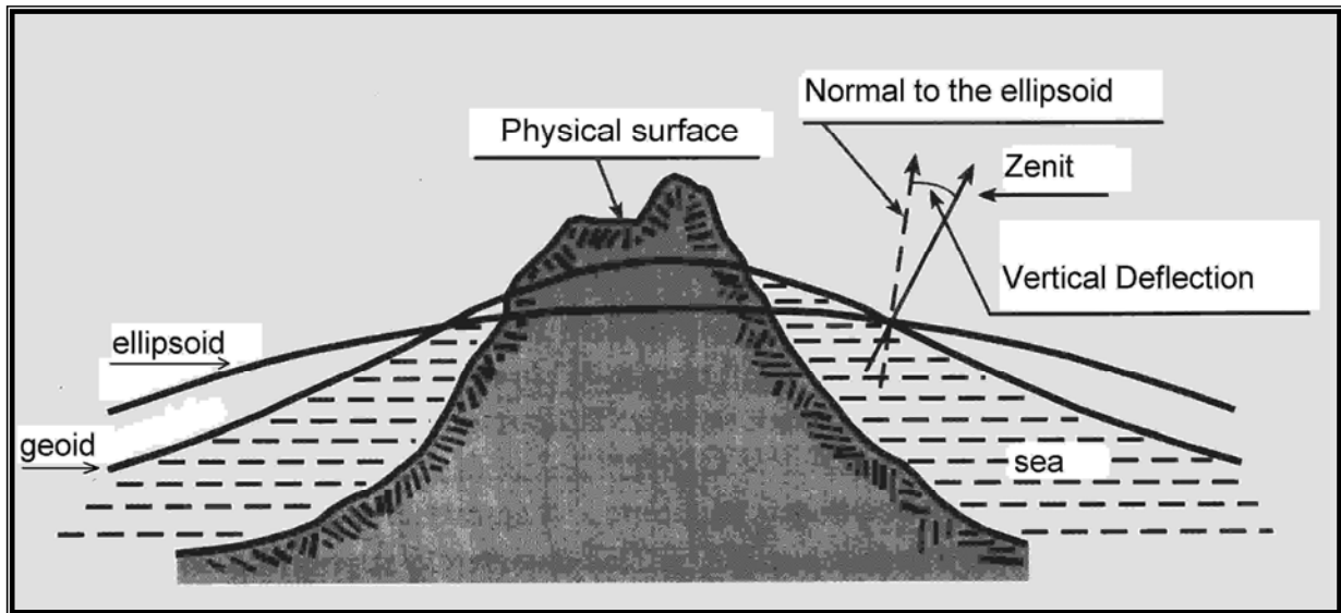
Fig. 2.1 "The Earth"
