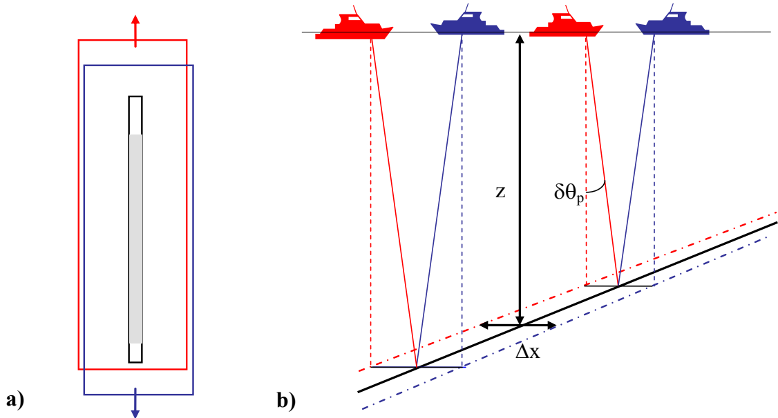
Fig. 3.37 "Pitch offset calibration.
