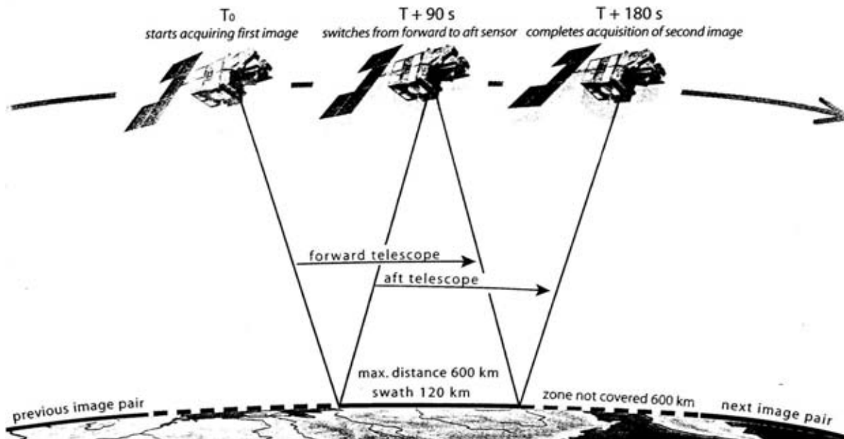
Fig. 6.54 "HRS SPOT-5 stereo geometry (after SPOT IMAGE, 2002)"
