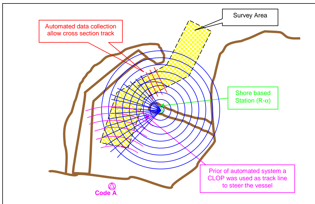
Fig. 7.6 “Range-Azimuth positioning”
