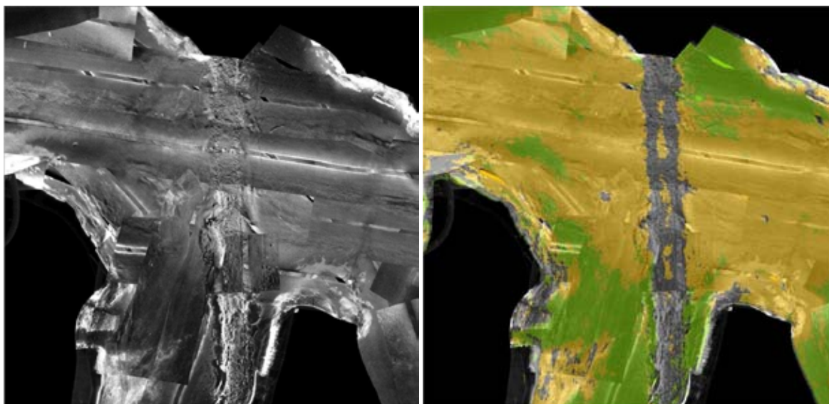
Fig. 4.8 Example of Sidescan Sonar Mosaic and Classification Models (using QinetiQ ‘Classiphi’ software)
