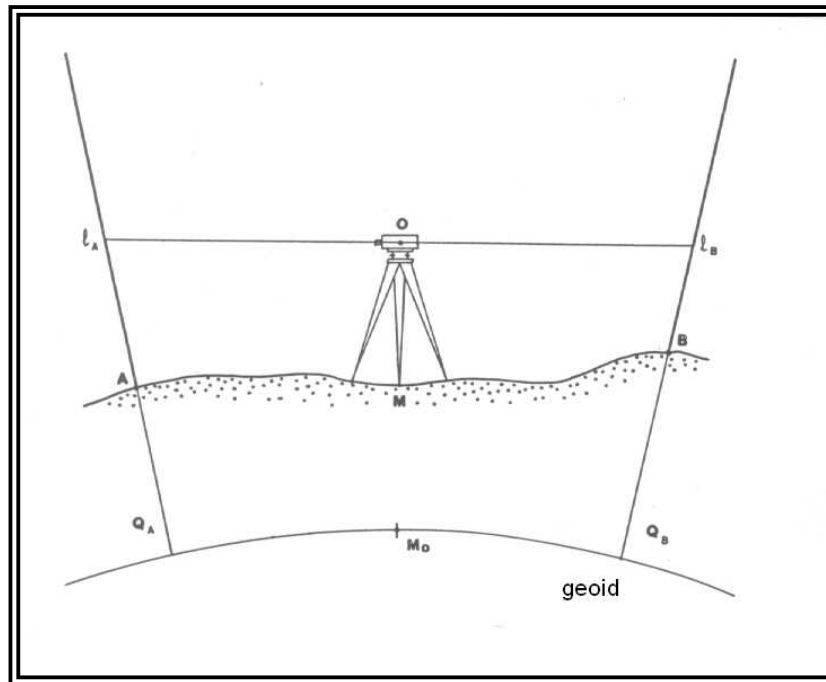
Fig. 2.15 “Geometric levelling”
