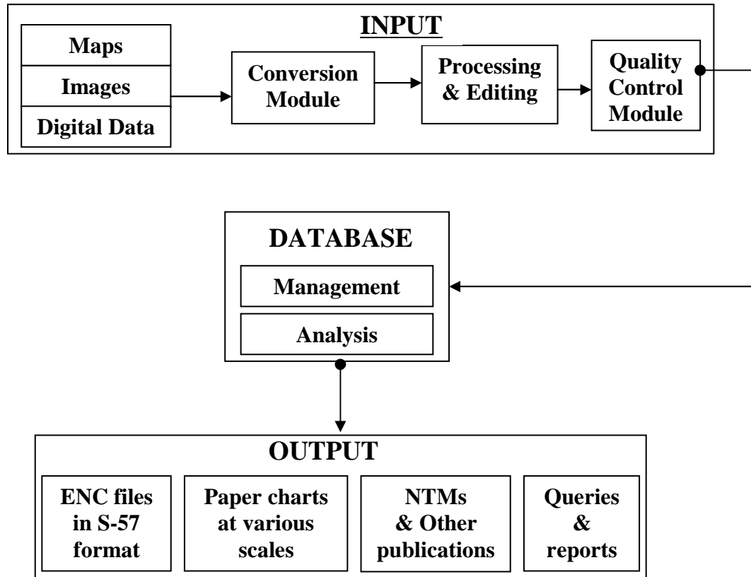
Fig. 1.3 "NIS Functional Subsystems"
