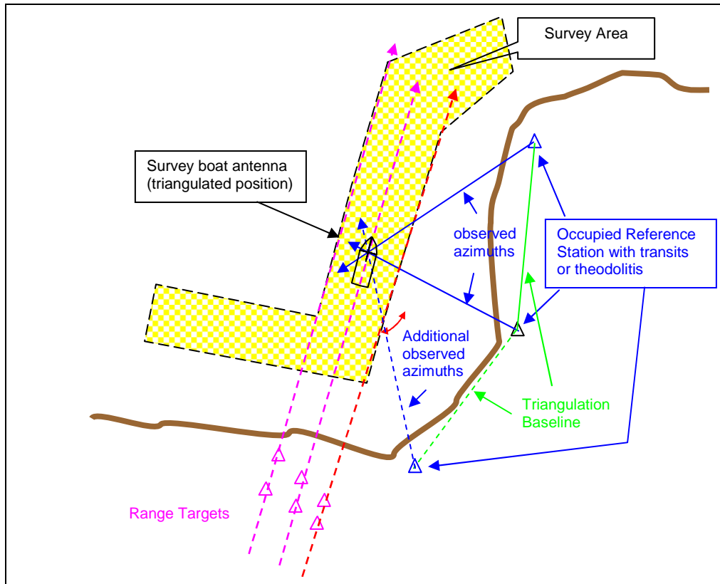
Fig. 7.3 “Triangulation/Intersection positioning”
